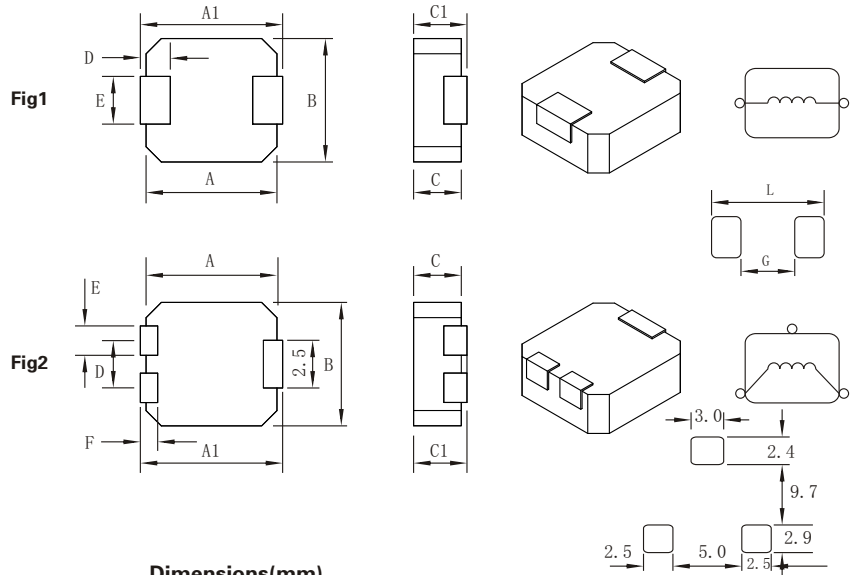
Dimensions(mm)
